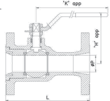
CLASS 300 FIG SV50301R
