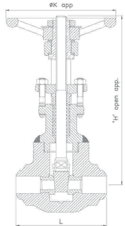
GATE VALVE FIG SVF1150 - SVF1250
