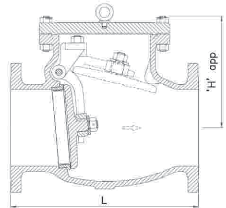
CLASS 150 FIG SV4015
