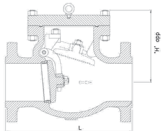
CLASS 600 FIG SV4060
