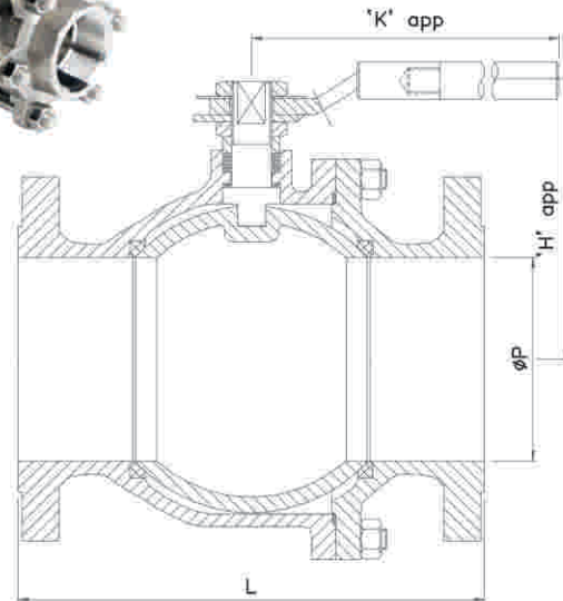
CLASS 150/300 2PIECE FIG SV50152F
