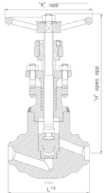
GLOBE VALVE FIG SVF2150 - SVF2250
